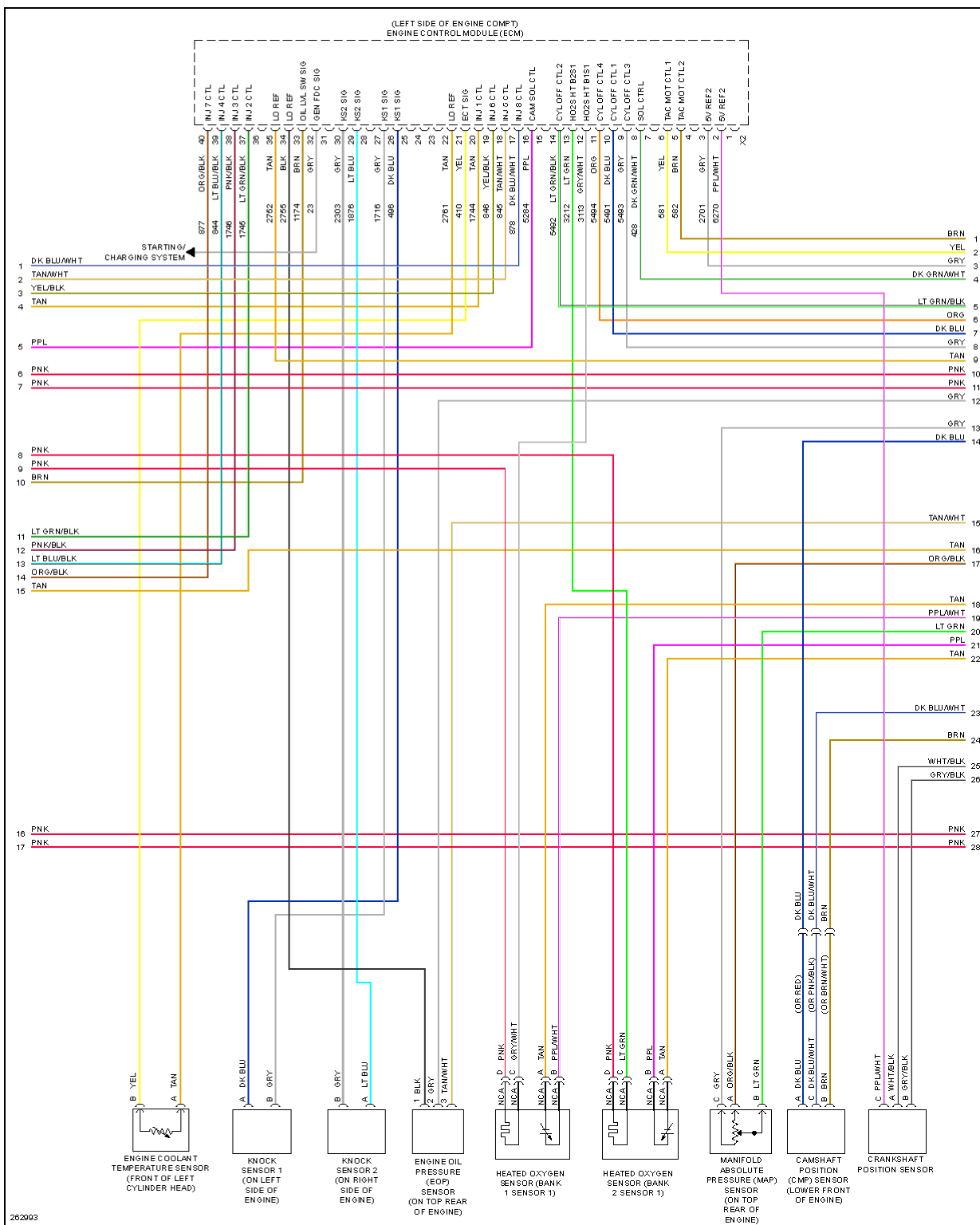
Fig. 28: 6.2L VIN 8, Engine Performance Circuit (4 of 5)
