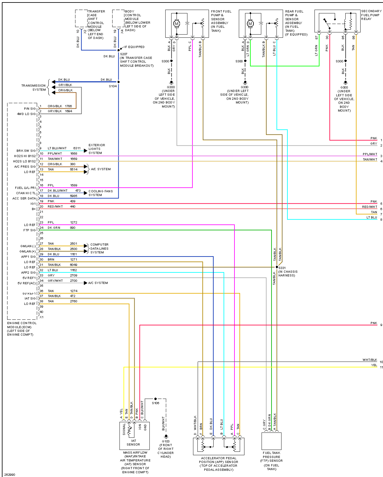
Fig. 25: 6.2L VIN 8, Engine Performance Circuit (1 of 5)
