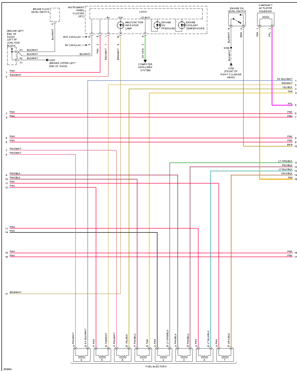
Fig. 27: 6.2L VIN 8, Engine Performance Circuit (3 of 5)
