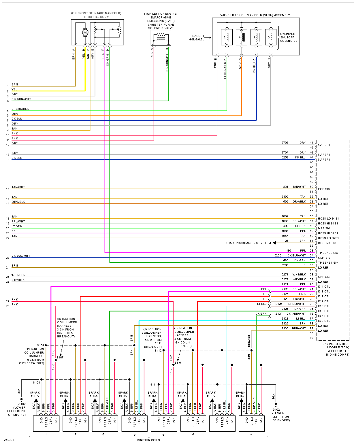
Fig. 29: 6.2L VIN 8, Engine Performance Circuit (5 of 5)
